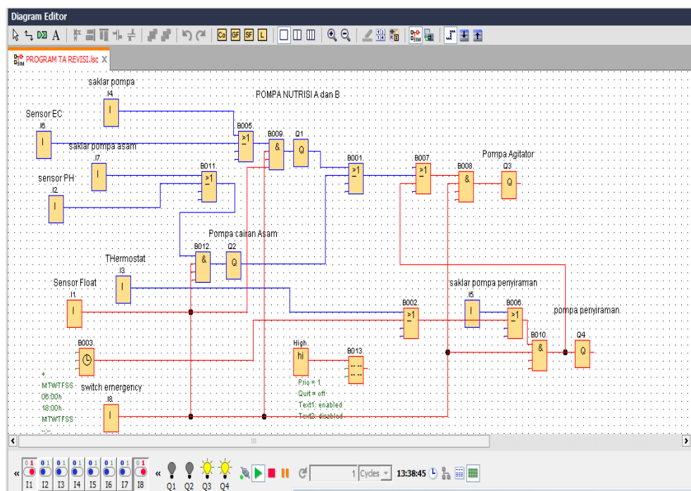
Gambar 4 Hasil pengujian simulasi LOGO!Soft Comfort V8.0
